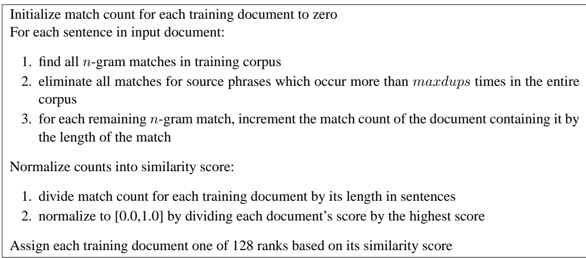
Figure 1: Similarity-scoring procedure
