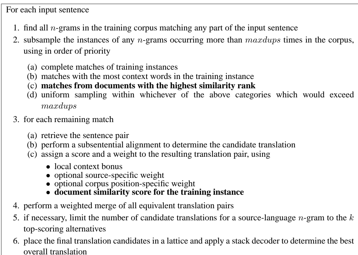
Figure 2: Translation process in pseudo-code
