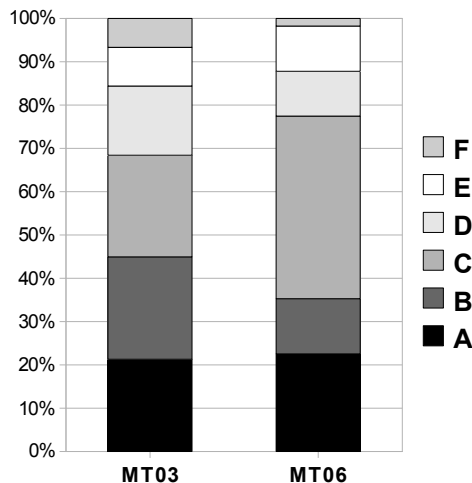
Figure 3: Contribution of each system to the new first best of the combination with all six systems for MT03 and MT06
